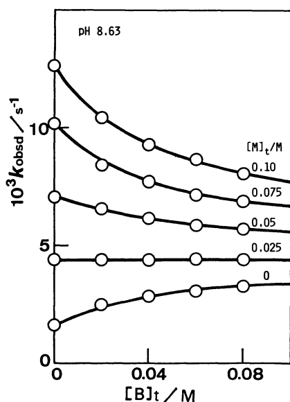
Fig. 5. Dependences of k_{\text{obsd}} on the concentration of boric acid at the concentrations of morpholine indicated.
